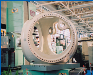
MACHINING OF WIND POWER GENERATOR
